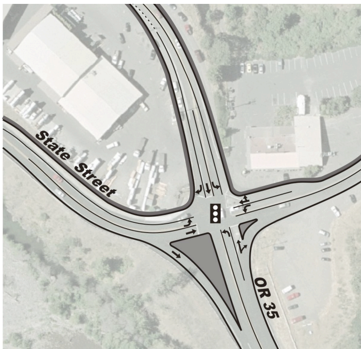
Figure 8: Recommended Improvements at OR 35 / State St.
